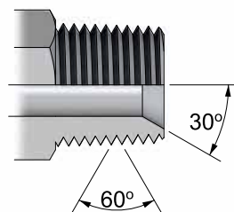
NPTF male (taper)
